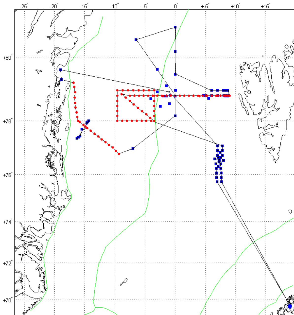
Fig. 1: Planned cruise track. The blue squares indicated the moorings and OBSs to be deployed and CTD stations are exemplarily marked by red dots. The exact locations for the deployments and CTD stations may deviate from the currently planned ones depending on the sea ice conditions during the cruise and the bathymetry.
