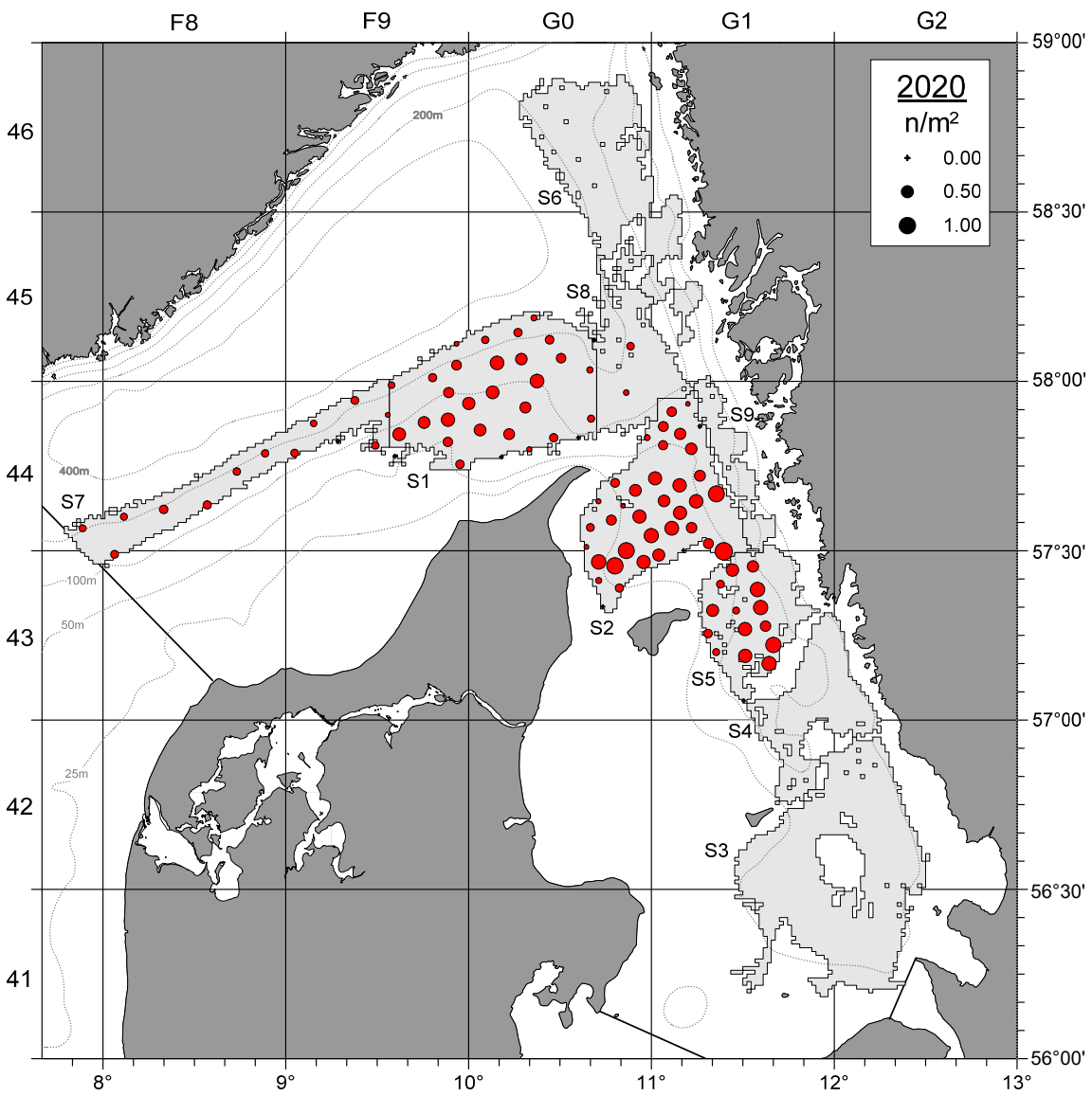
Figur 2. Antal jomfruhummerhuller per m 2 , UWTV Monitoring 2020 Danmark.
